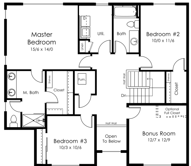
■ Upper Floor 1310 SF
