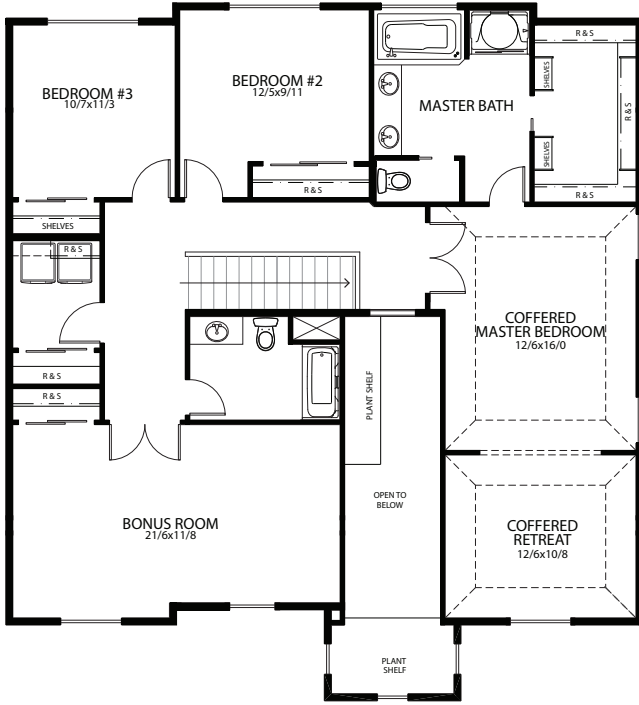
SECOND FLOOR 1525 SQ. FT.
